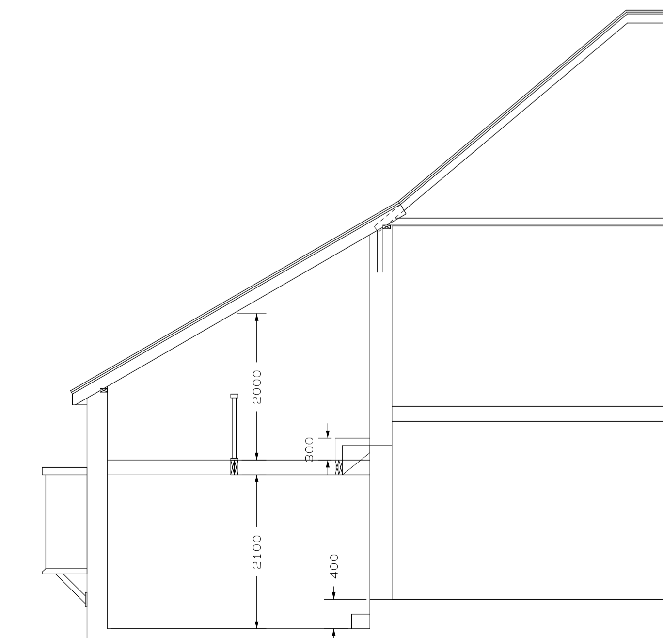
SECTION THROUGH 1:50
